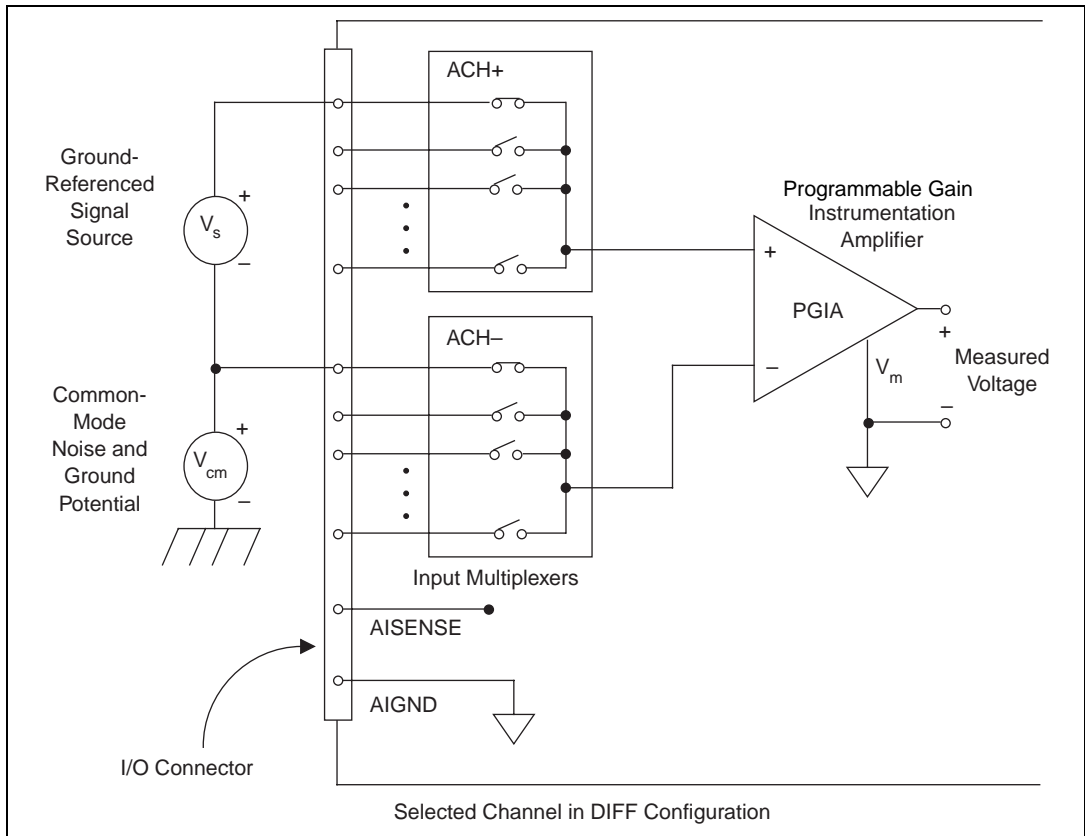
Figure 4-7. Single-Ended Input Connections for Ground-Referenced Signals
