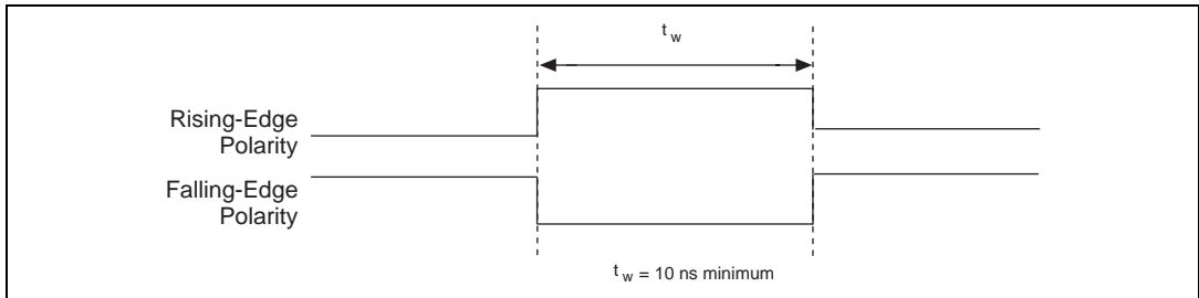
Figure 4-30. GPCTR0_GATE Signal Timing in Edge-Detection Mode
