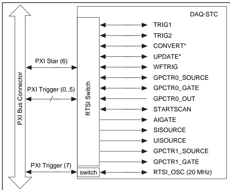
Figure 3-4. PXI RTSI Bus Signal Connection
