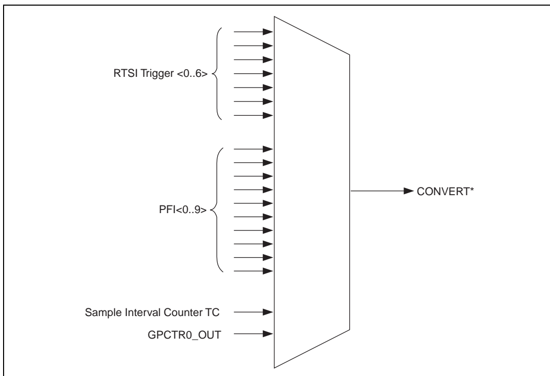
Figure 3-2. CONVERT* Signal Routing
