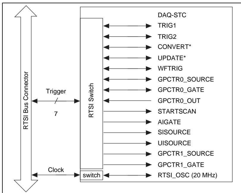
Figure 3-3. PCI RTSI Bus Signal Connection
