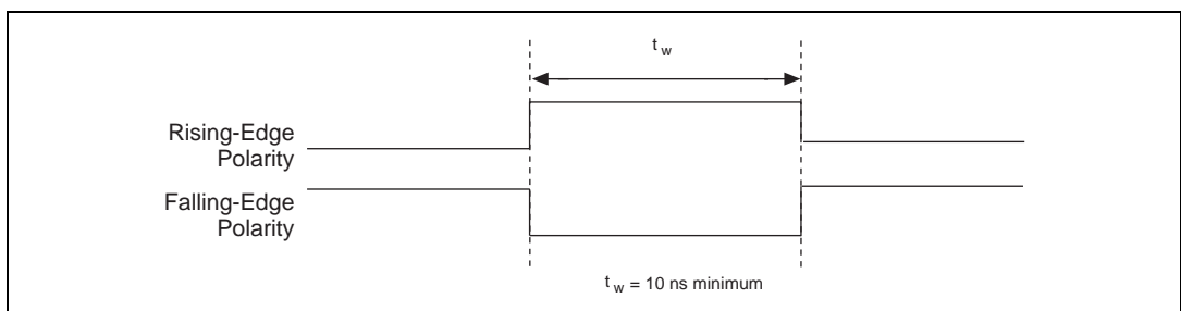
Figure 4-17. TRIG2 Input Signal Timing
