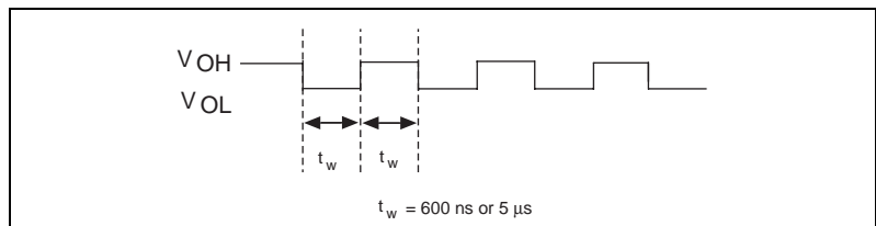
Figure 4-14. EXTSTROBE* Signal Timing
