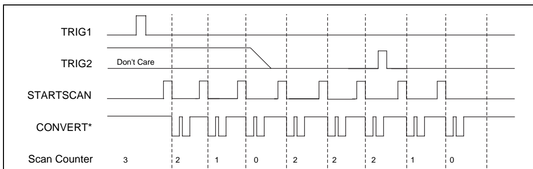
Figure 4-12. Typical Pretriggered Acquisition
