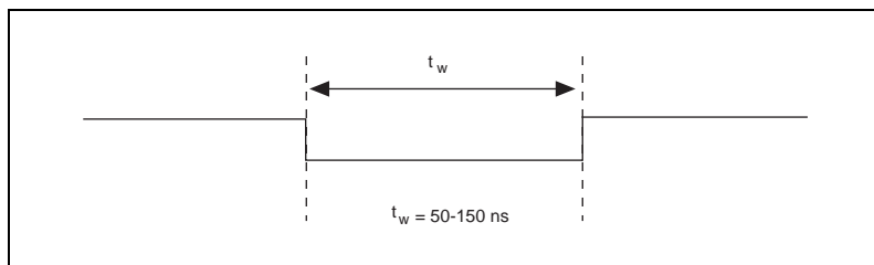
Figure 4-22. CONVERT* Output Signal Timing
