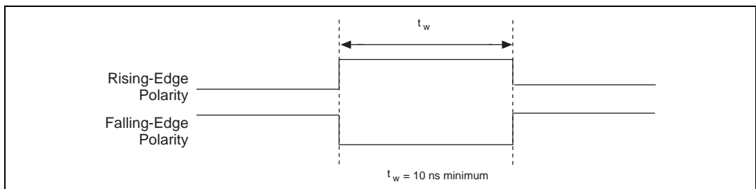
Figure 4-33. GPCTR1_GATE Signal Timing in Edge-Detection Mode
