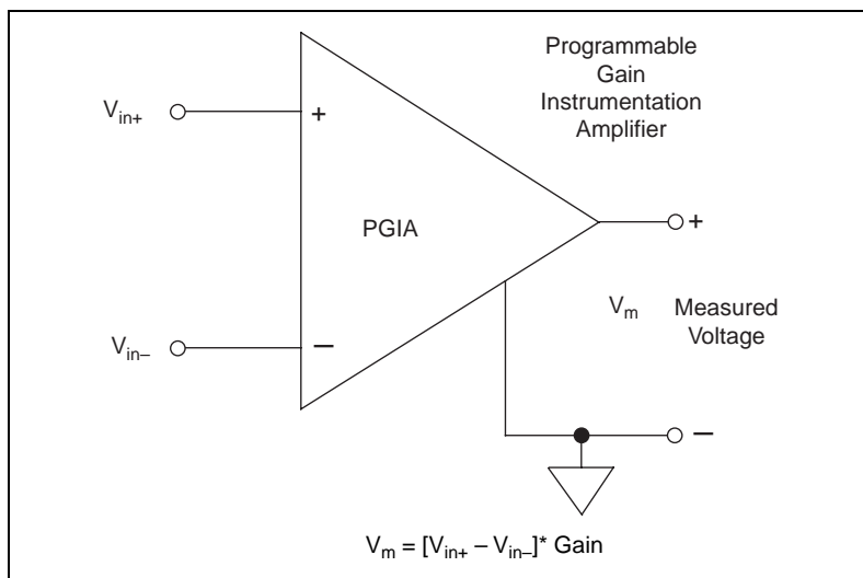
Figure 4-2. Programmable Gain Instrumentation Amplifier (PGIA)
