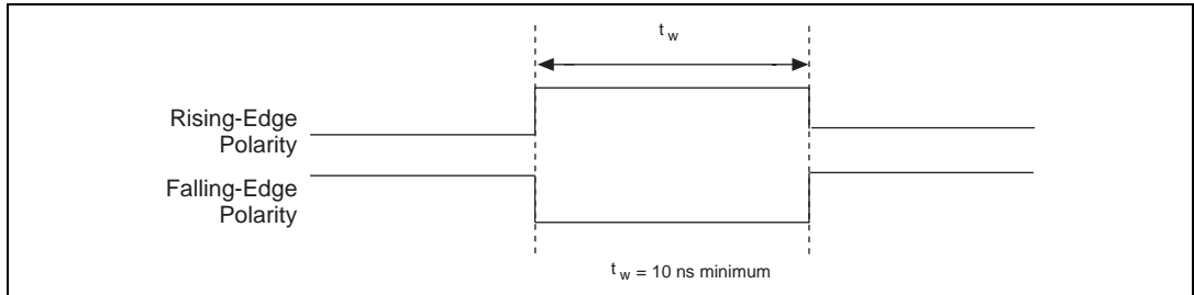
Figure 4-24. WFTRIG Input Signal Timing
