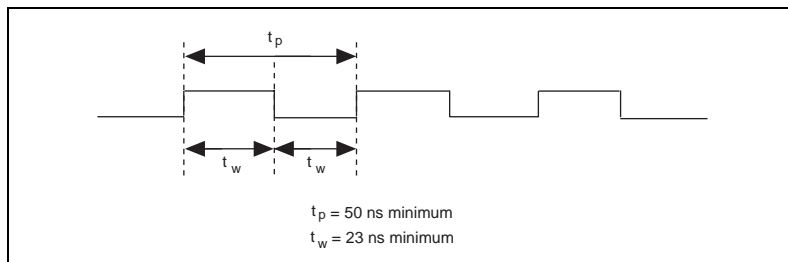
Figure 4-29. GPCTR0_SOURCE Signal Timing
