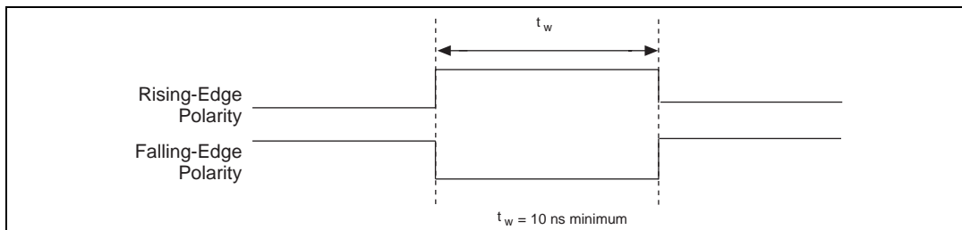
Figure 4-19. STARTSCAN Input Signal Timing
