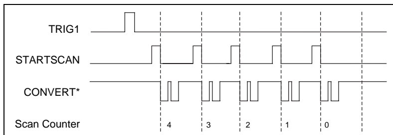
Figure 4-11. Typical Posttriggered Acquisition
