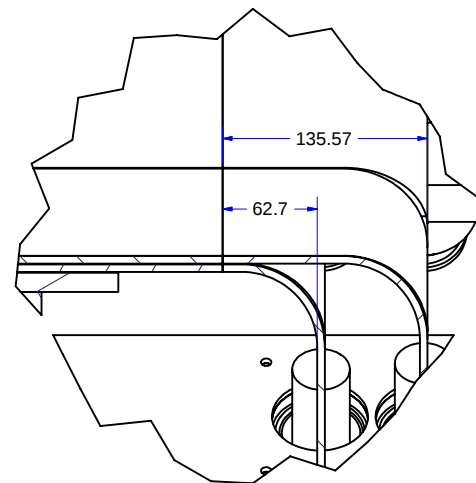
DETAIL E SCALE 0.40 : 1
